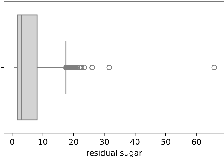
Box-plot Incondicional - residual sugar
